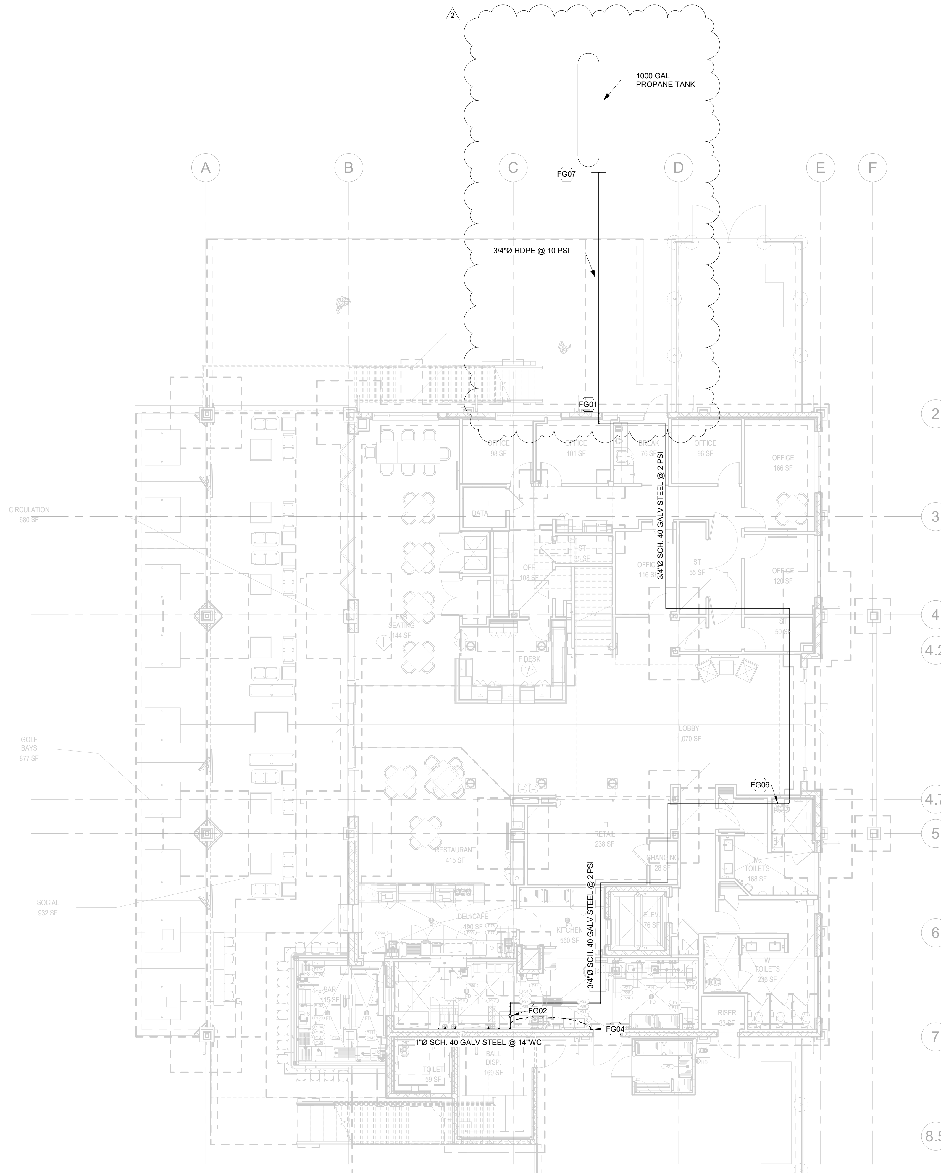
OVERALL FUEL GAS PLAN - FIRST FLOOR 1/8" = 1'-0"
